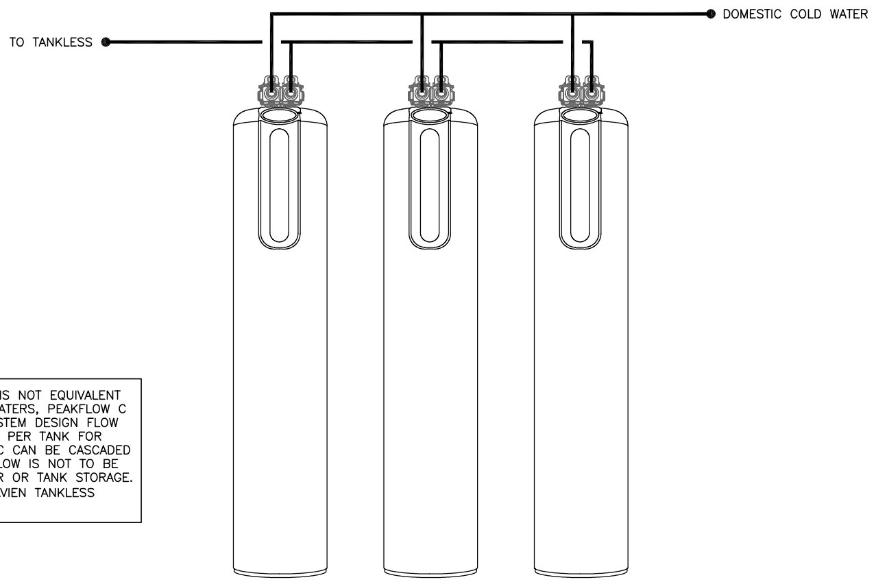
FRONT VIEW
