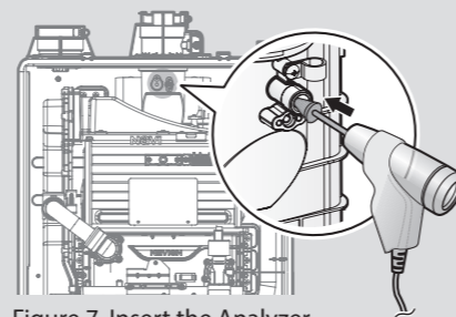
Figure 7. Insert the Analyzer
