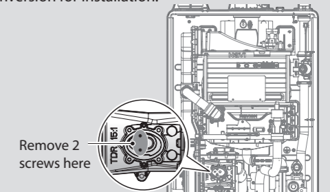
Figure 4. Access to Gas Orifice in Fan Assembly
